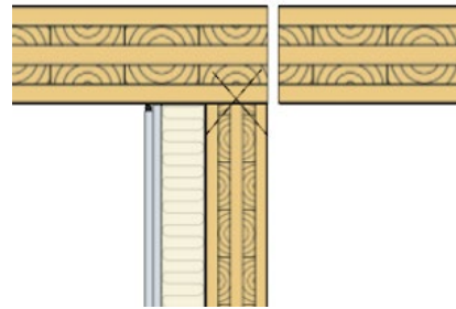
Figure 7: Drawing of vertical cross section displaying the junction between horizontally adjacent rooms.
