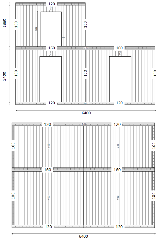
Figure 2: Vertical section drawings of the test mock-up; a) length section and b) width section. All dimensions are given in mm.
