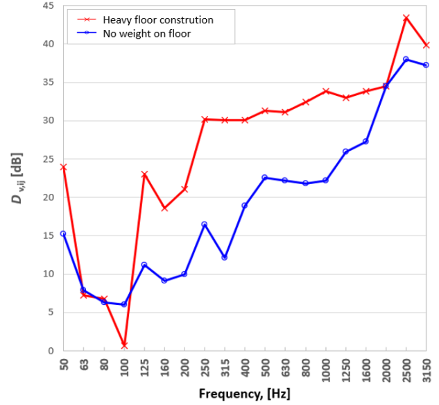
Figure 9: Measurement results with (red line) and without (blue line) heavy floor construction.
